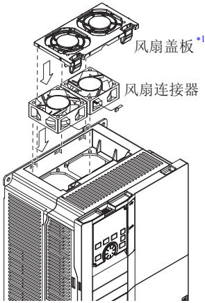
FR-A820-00340 (5.5K) ～ FR-A820-01540 (30K) FR-A840-00170 (5.5K) ～ FR-A840-00770 (30K)
